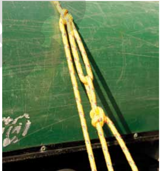
Secure the kayak to the racks using cam straps, bungee cords, or lines using a trucker's hitch. The lines should be tight and secure, but be careful: It is possible to tighten hard enough to damage the hull.
